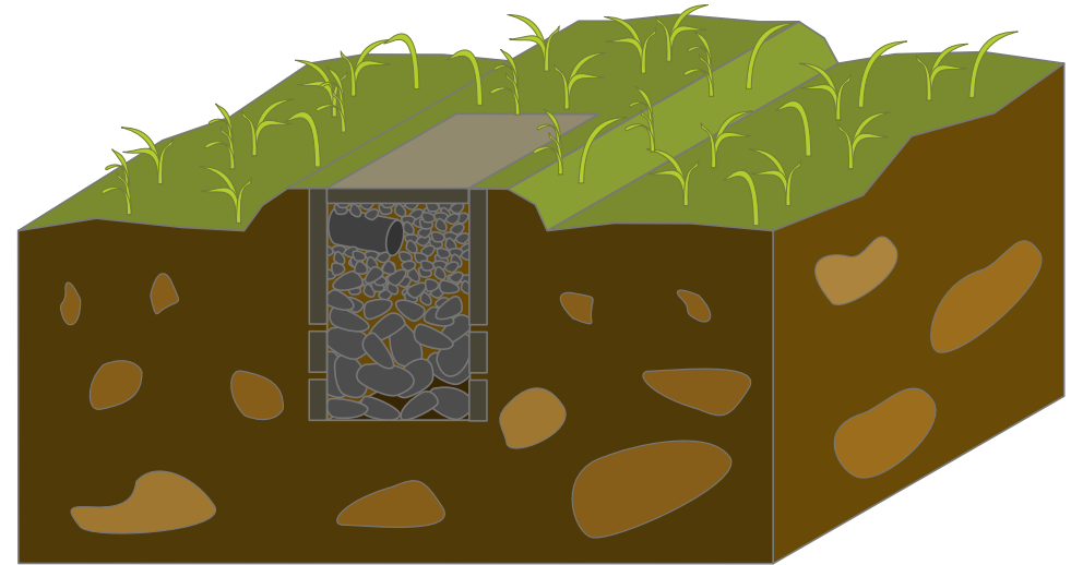
A potential type of dry well. The water from above going into the well generally seeps through holes in the walls or by the bottom of the well. Basic models with natural materials can also be efficient (see the diagram with a trench filled with stones in the part “VII.2.3. Drainage”).
