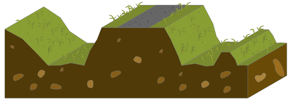
From left to right, a slope, then a levee (here equipped with a pathway). The levee is a security that blocks important amounts of water. On the right, the mound which has the same goal as the levee, but for much smaller amounts of water.
