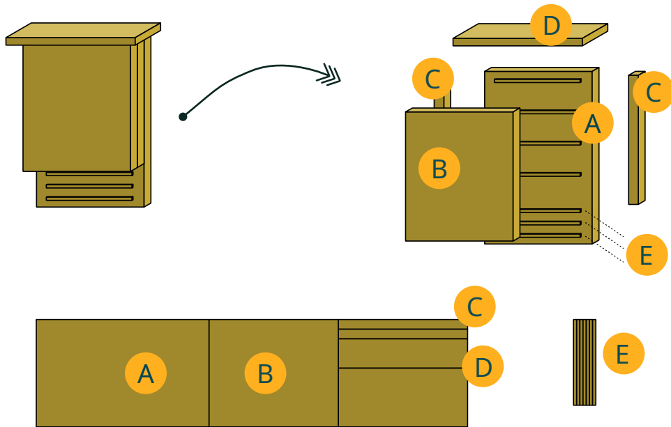
Exploded view of a bat shelter (thereafter, the values are inspired by the LPO Auvergne-Rhône-Alpes association).
