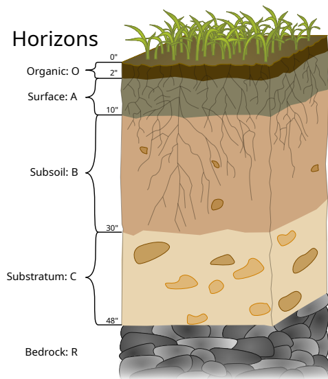
Illustration of the soil horizon (by "Wilsonbiggs", CC BY SA license).
