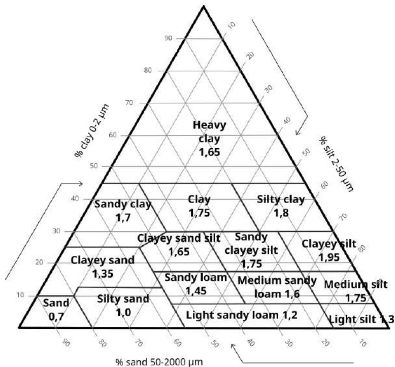
Jamagne's Triangle of Textures (1977) with indication of the available water capacity (AWC) in mm/cm
